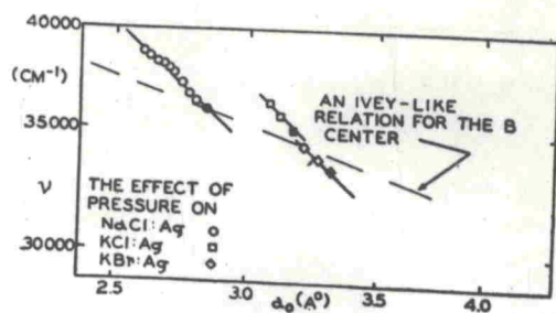
FIG. 8. An Ivey-like relation for the B center, and the compressibility near a B center.
